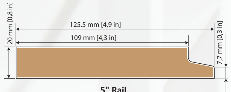
5" Rail
