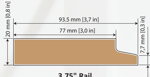
3.75" Rail
