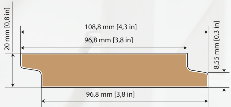
4.5" Divider
