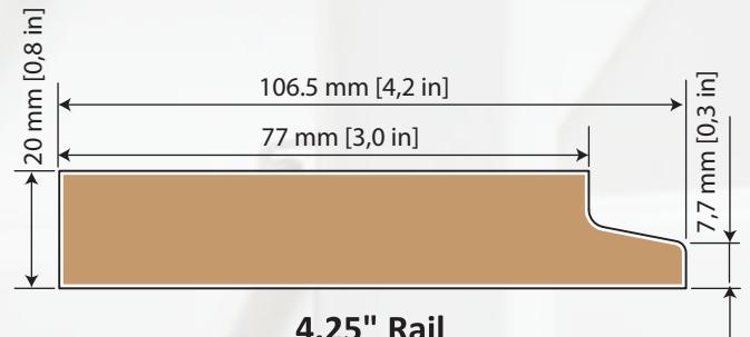
4.25" Rail
